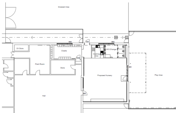
Proposed Floor Plan Holy Trinity Rosehill VA CE Primary, Stockton
