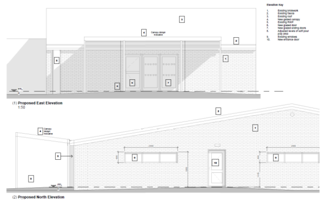
(2) Proposed North Elevation 1:50
